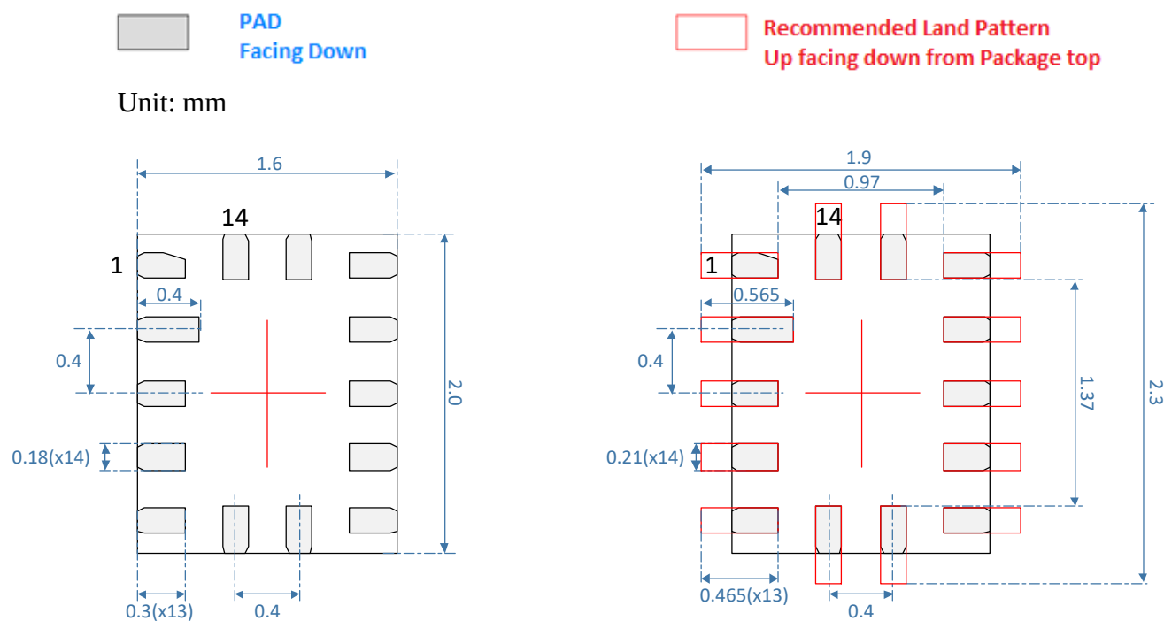
图 35: Recommended Land Pattern
